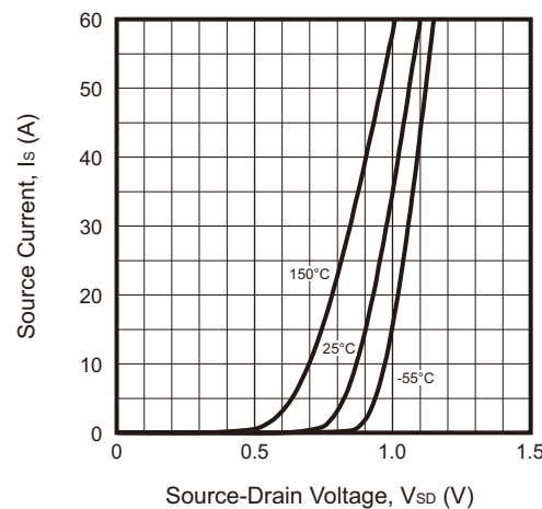
Fig.6 - Body-Diode Characteristics
